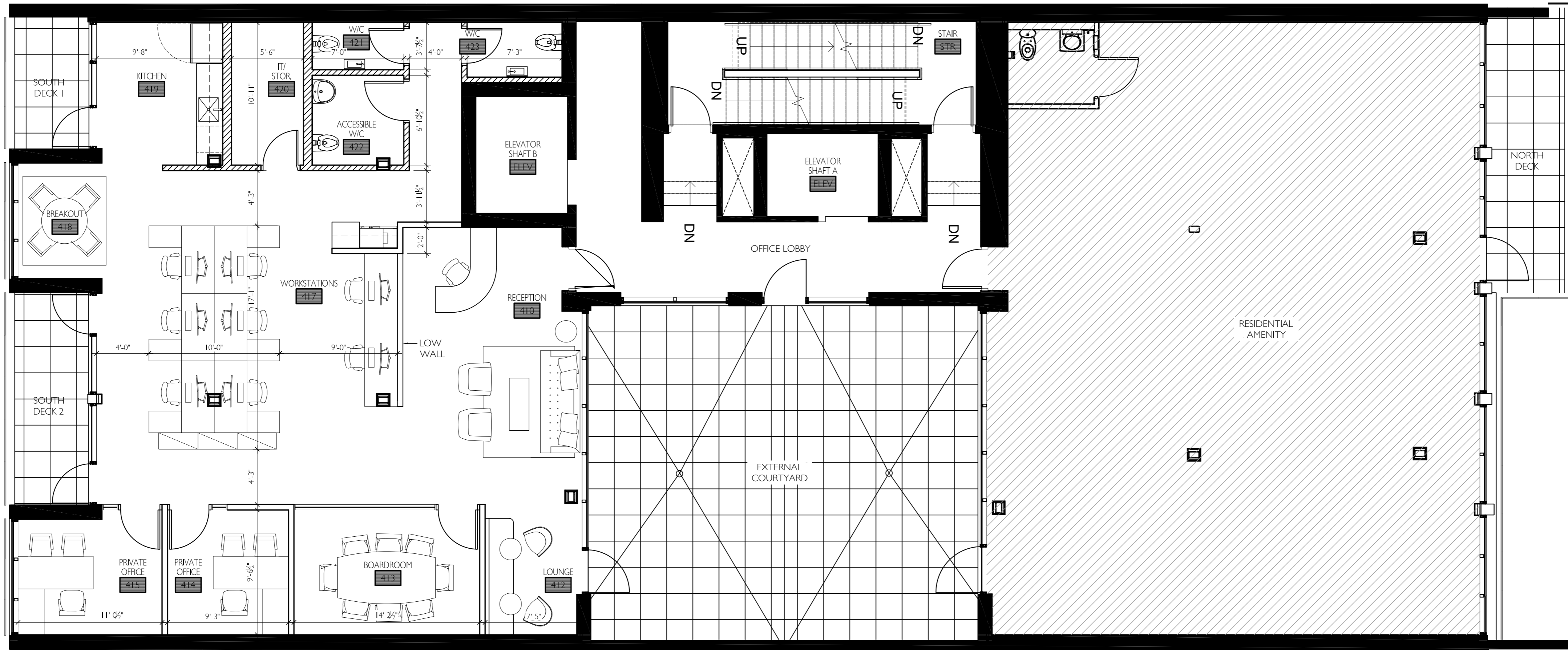
1 SPACE PLAN - 3RD FLOOR | 1724 SQ FT 3/8" = 1'-0"
