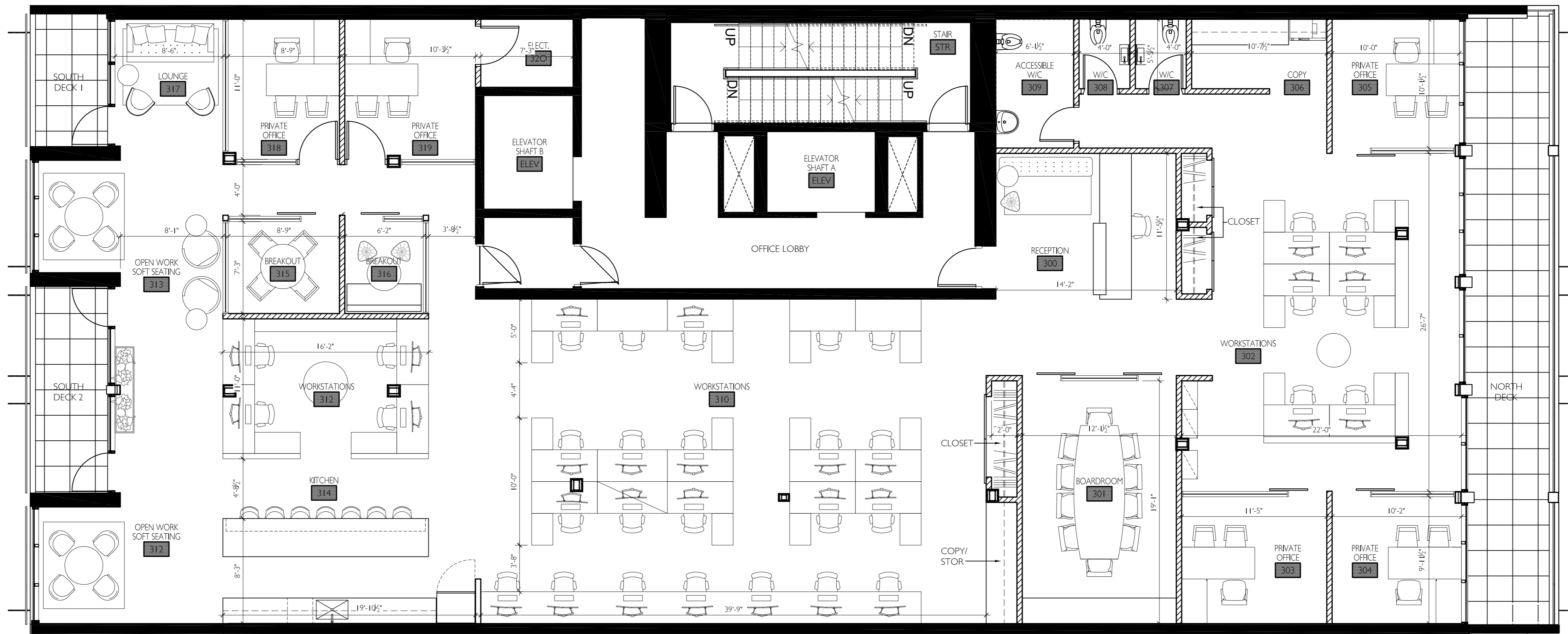
1 SPACE PLAN - 2ND FLOOR | 4267 SQ FT 3/8" = 1'-0"
